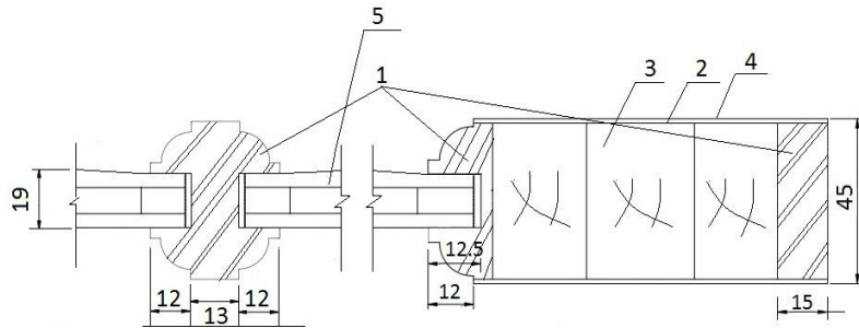
PROFILE B-B
